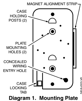
Diagram 1. Mounting Plate
